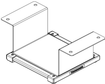
CPU Bracket
